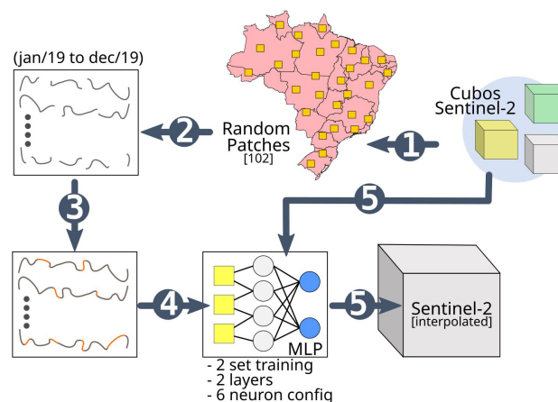
Figure 1: The methodological scheme used in this study, with the main tasks: 1-random points generation; 2-extraction of the time series; 3-linear interpolation; 4-training the MLP model; 5-predicting the cloud-free values for a year of images.
